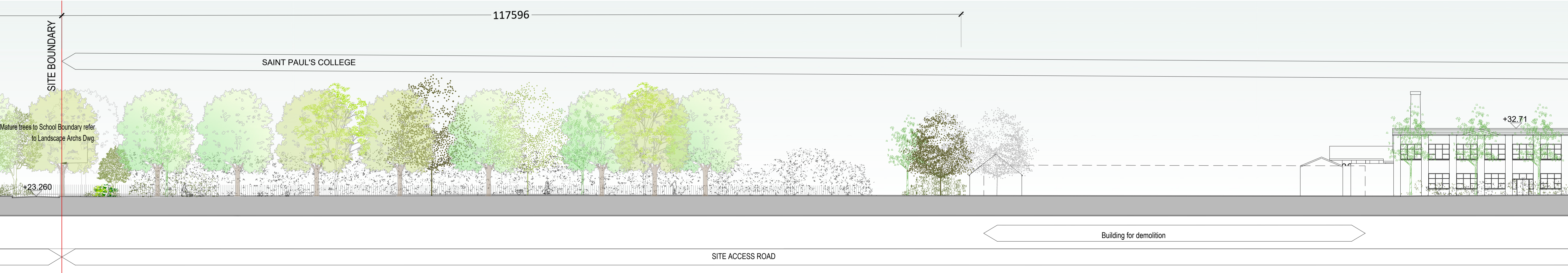
SITE SECTION B-B (PART 2) 1/250
